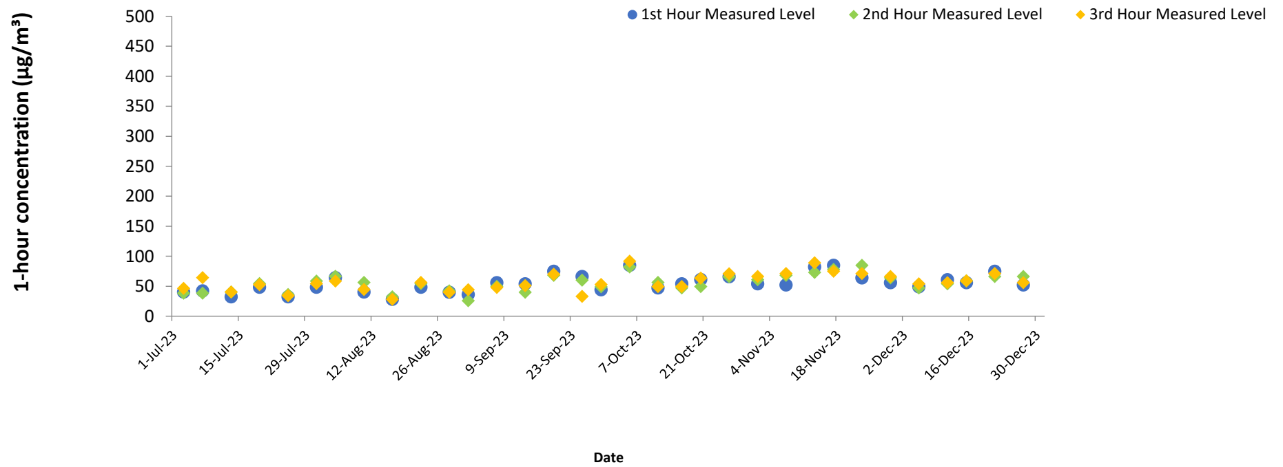
1-hour TSP concentration vs date for Location M-A3
